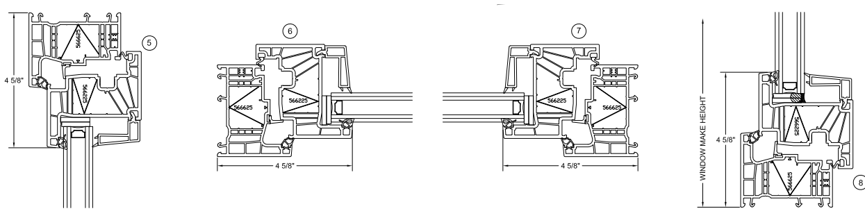
Casement/Casement Detail
