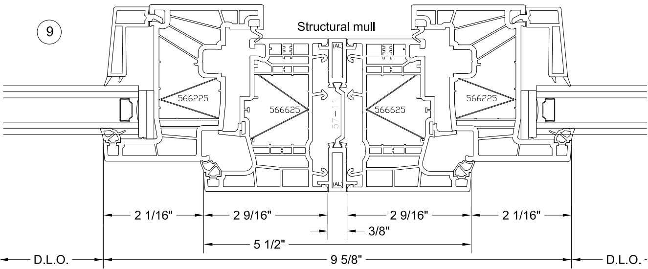
Casement/Casement Detail
