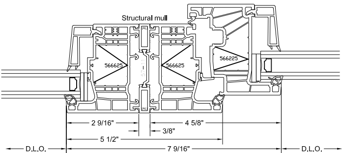
Fixed/Casement Detail
