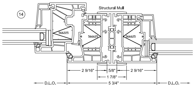
Casement/Fixed Detail
