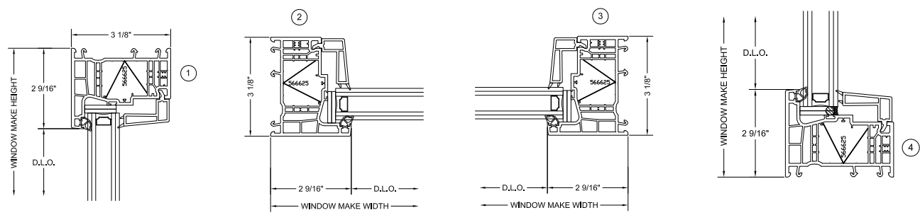
Fixed/Fixed Detail
