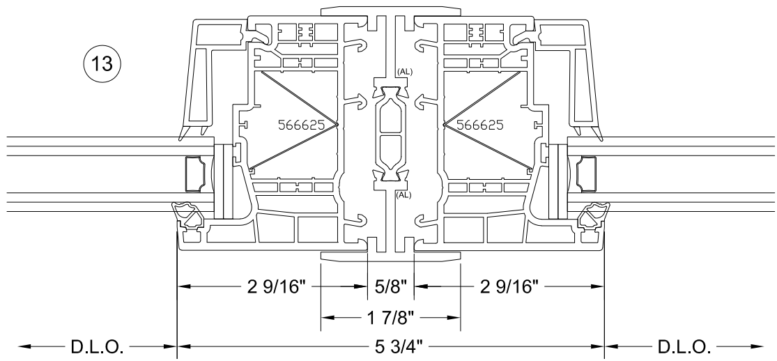
Fixed/Fixed Detail
