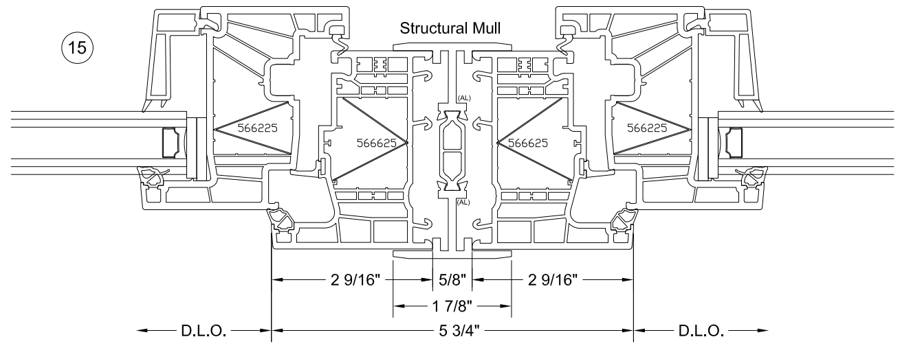
Casement/Casement Detail
