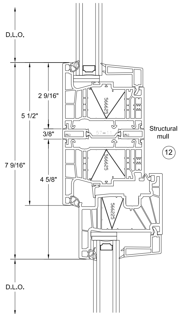
Fixed Over Casement Detail
