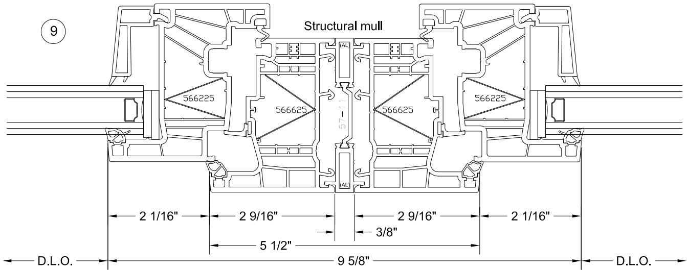
Casement / Casement Detail
