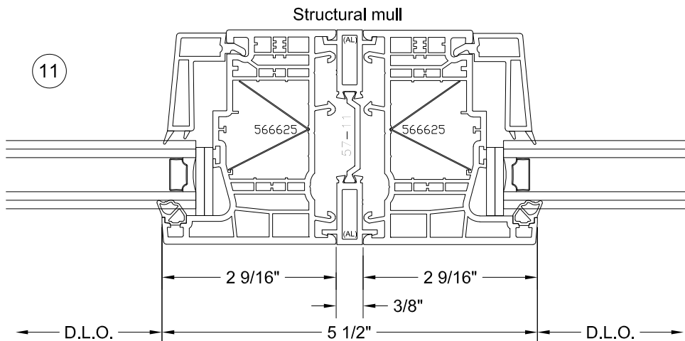
Fixed / Fixed Detail
